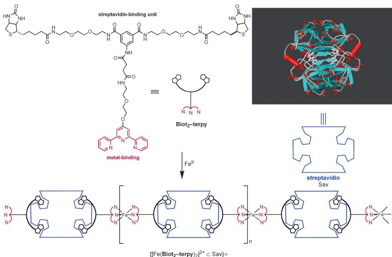
Figure 2. Structure of the bis-biotinylated (black) terpyridine (violet) Biot 2 -terpy, which, upon reaction with Fe II , forms a linear tetrabiocinylated connector, the [\text{Fe}(\text{Biot}_2\text{-terpy})_2]^{2+} complex. In the presence of streptavidin (right insert emphasizing the 48 acidic side chains and the stick representation shown in red), [50] linear coordination polymers, [[\text{Fe}(\text{Biot}_2\text{-terpy})_2]^{2+} \subset \text{Sav}]_\infty , are formed.
